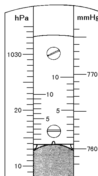
Figure 1.5 A vernier scale
